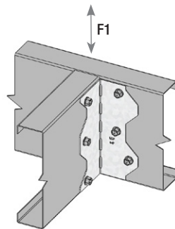
Typical MP/S7 installation (MP/S5 similar)
