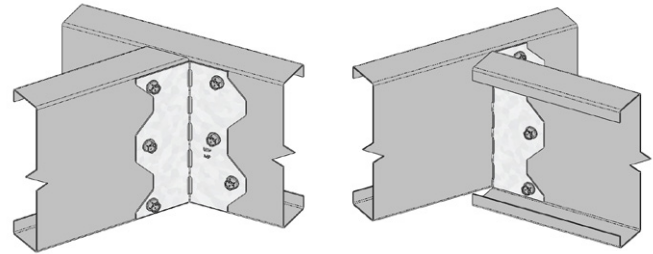
Typical MP/S7 skew installation (MP/S5 similar)
