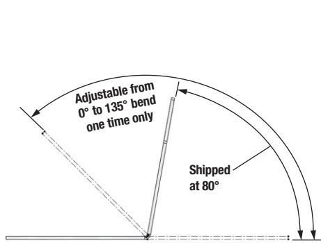
MP/S Top View
